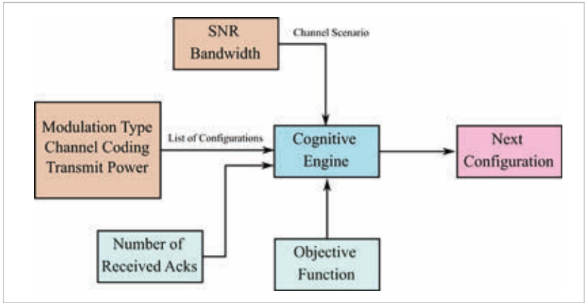
4. Shown is the cognitive radio framework implemented in Asadi et al [see Reference].
