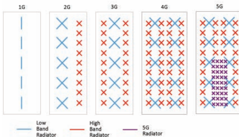
1. As mobile communications technology evolved from 1G to 4G and 5G, an increasing number of arrays of radiating elements within each generation of antenna has necessitated the technique of interleaving low- and high-band elements to avoid increasing antenna size. Images courtesy of Alpha Wireless
